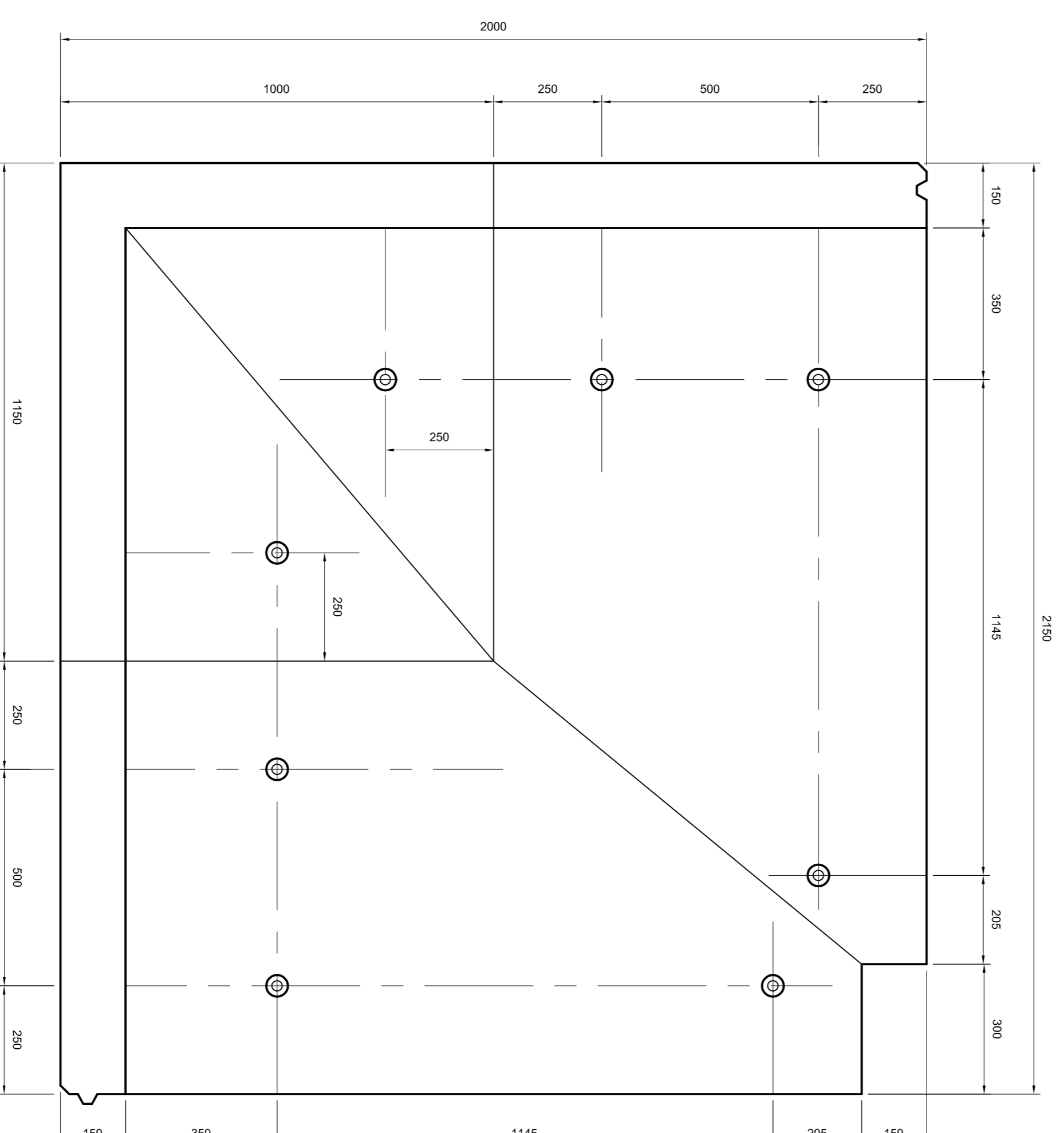
SECTION A-A PLAN ON ANCHOR BOLT SETTING OUT
