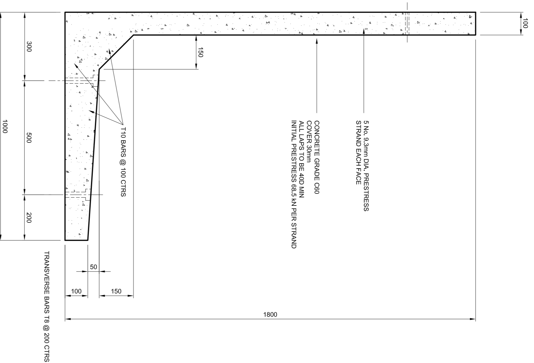
TYPICAL SECTION THROUGH 1800mm WALL UNIT 800 Kg PER 1800mm WALL UNIT
