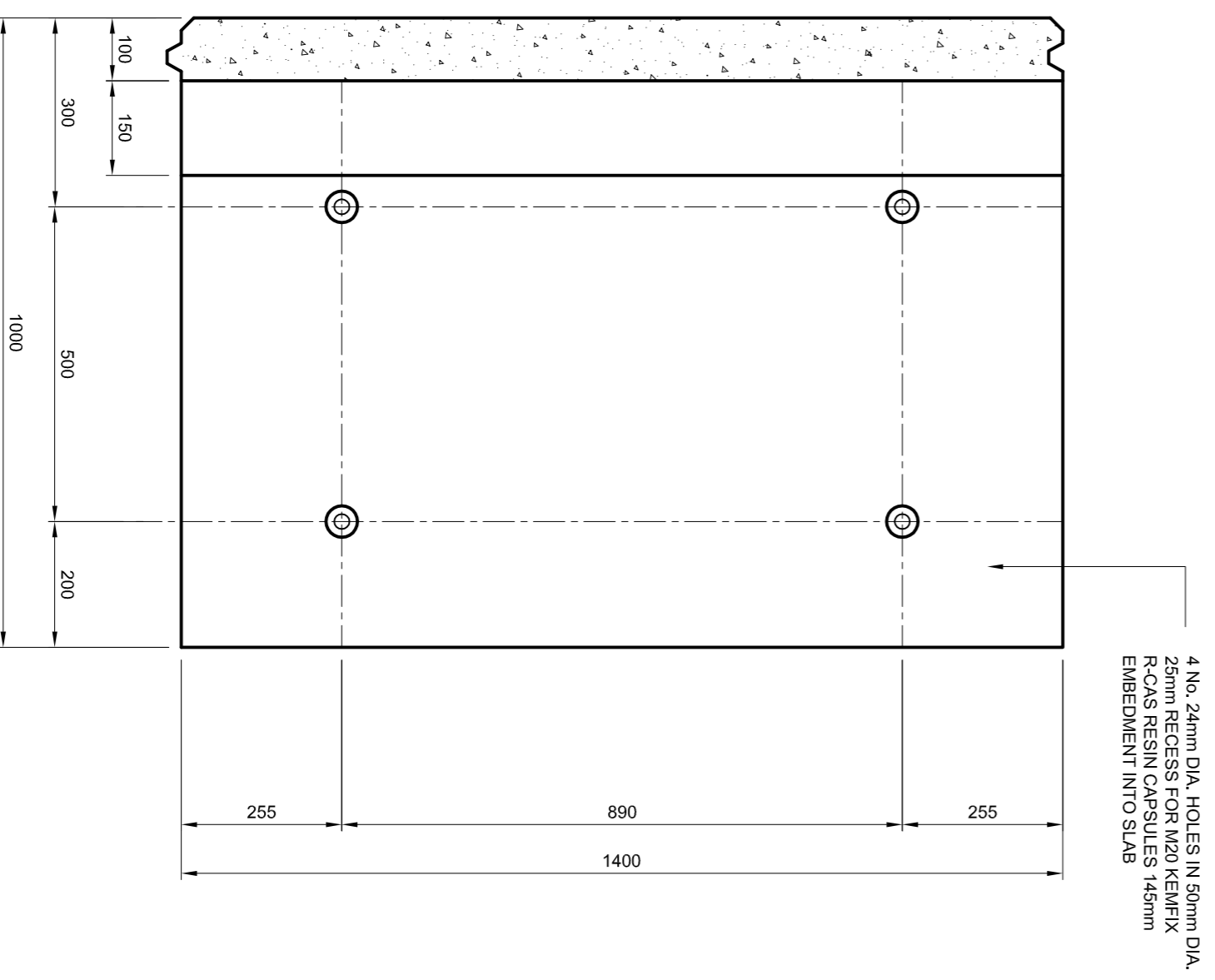
SECTION AA PLAN ON ANCHOR BOLT SETTING OUT
