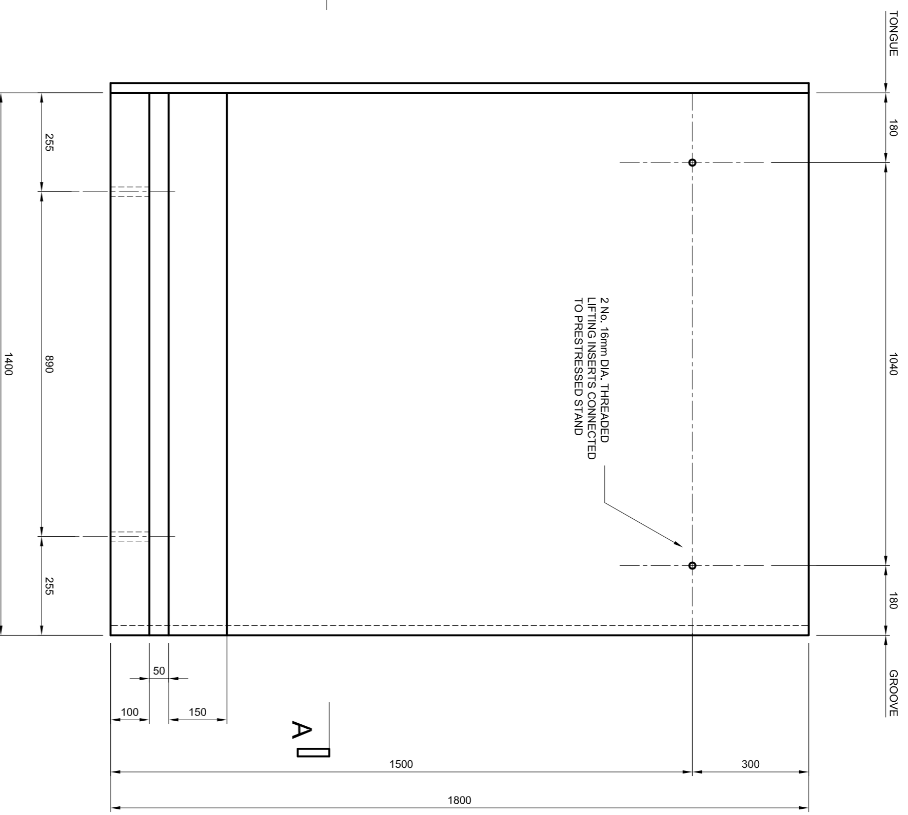
ELEVATION ON 1800mm WALL UNIT RC REMOVED FOR CLARITY
