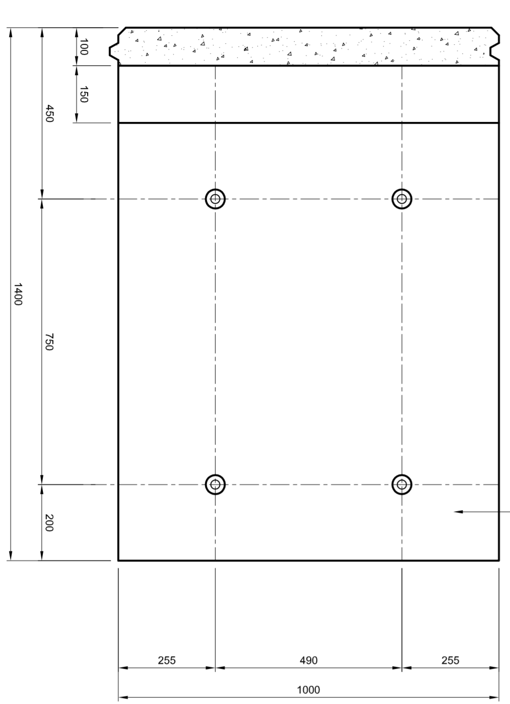
SECTION A-A PLAN ON ANCHOR BOLT SETTING OUT
