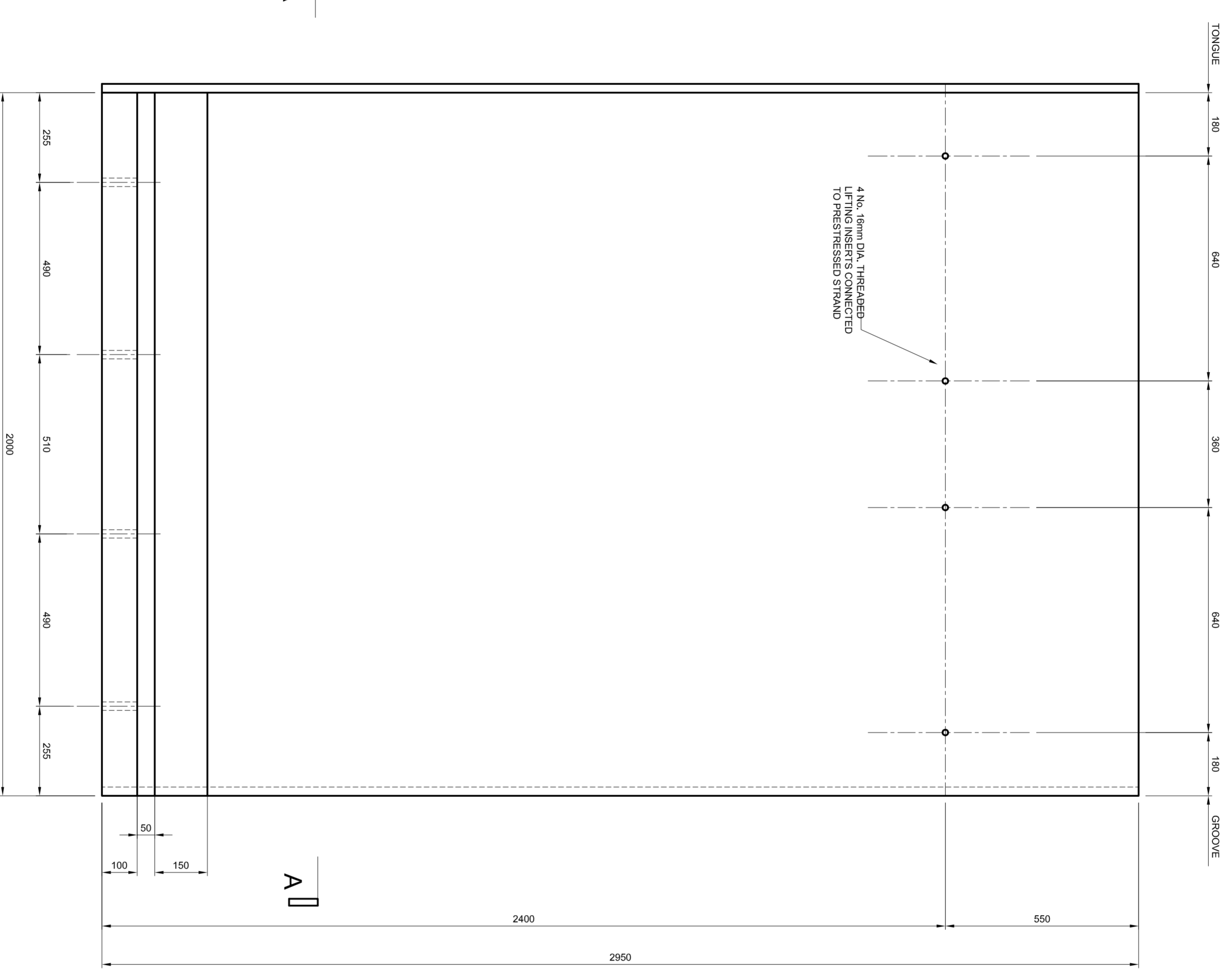
ELEVATION ON 2950mm WALL UNIT RC REMOVED FOR CLARITY
