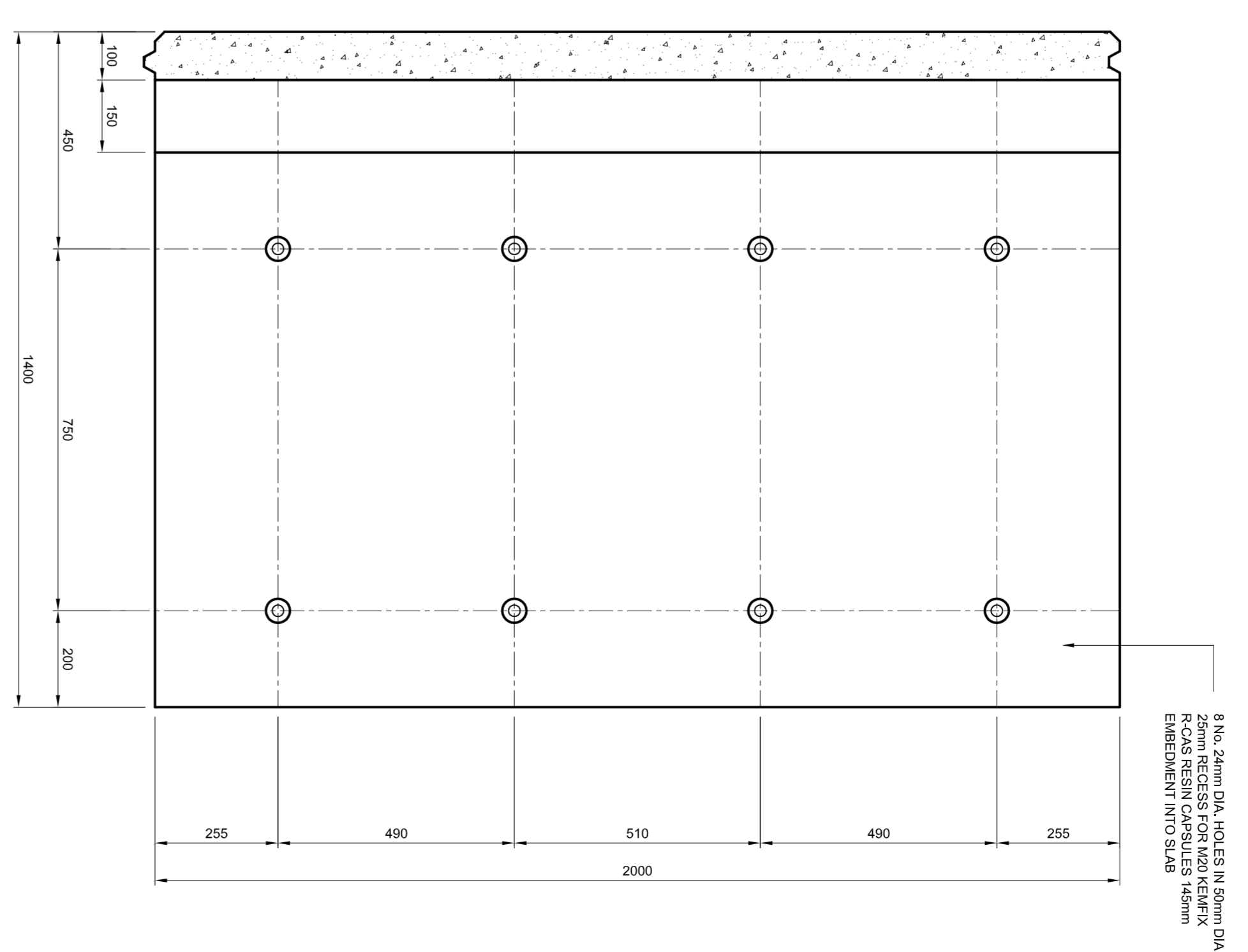
SECTION A-A PLAN ON ANCHOR BOLT SETTING OUT
