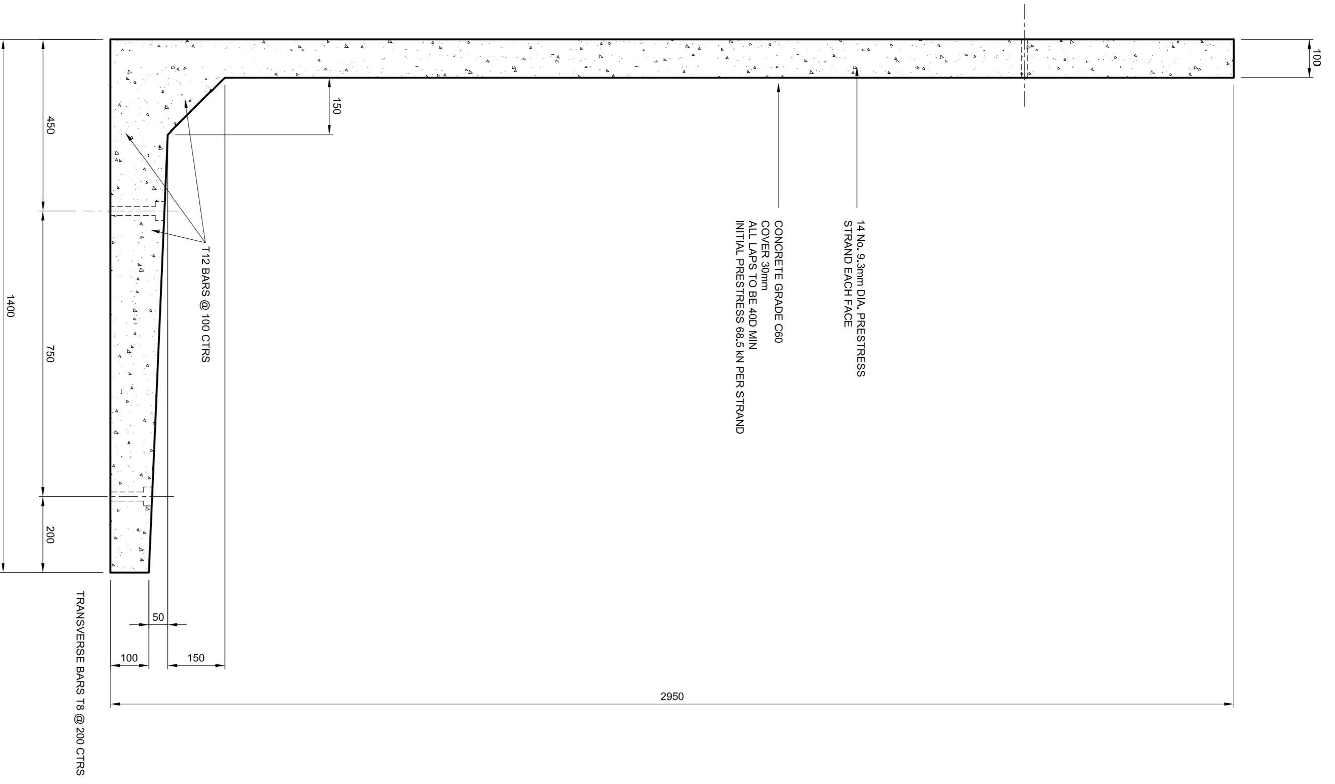
TYPICAL SECTION THROUGH 2950mm WALL UNIT
